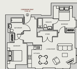
TYPE 13 71.8 - 72.0 m 2
